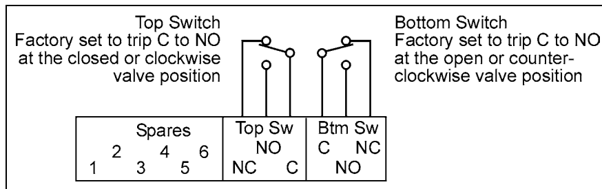
Figure 2—Proximity Switches
