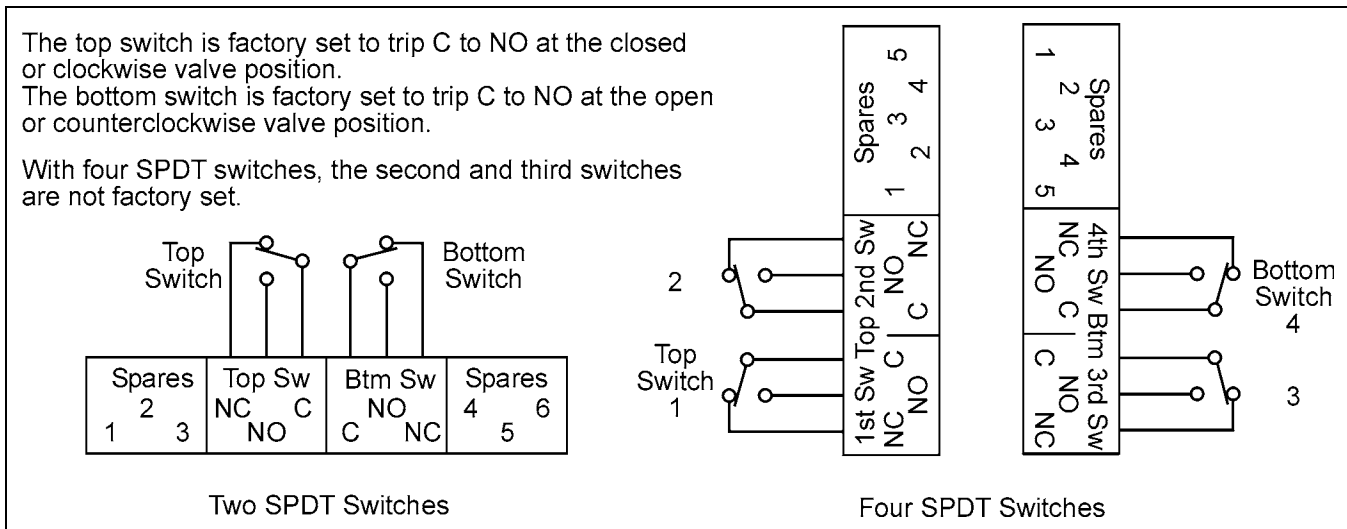
Figure 1— Mechanical Switches
