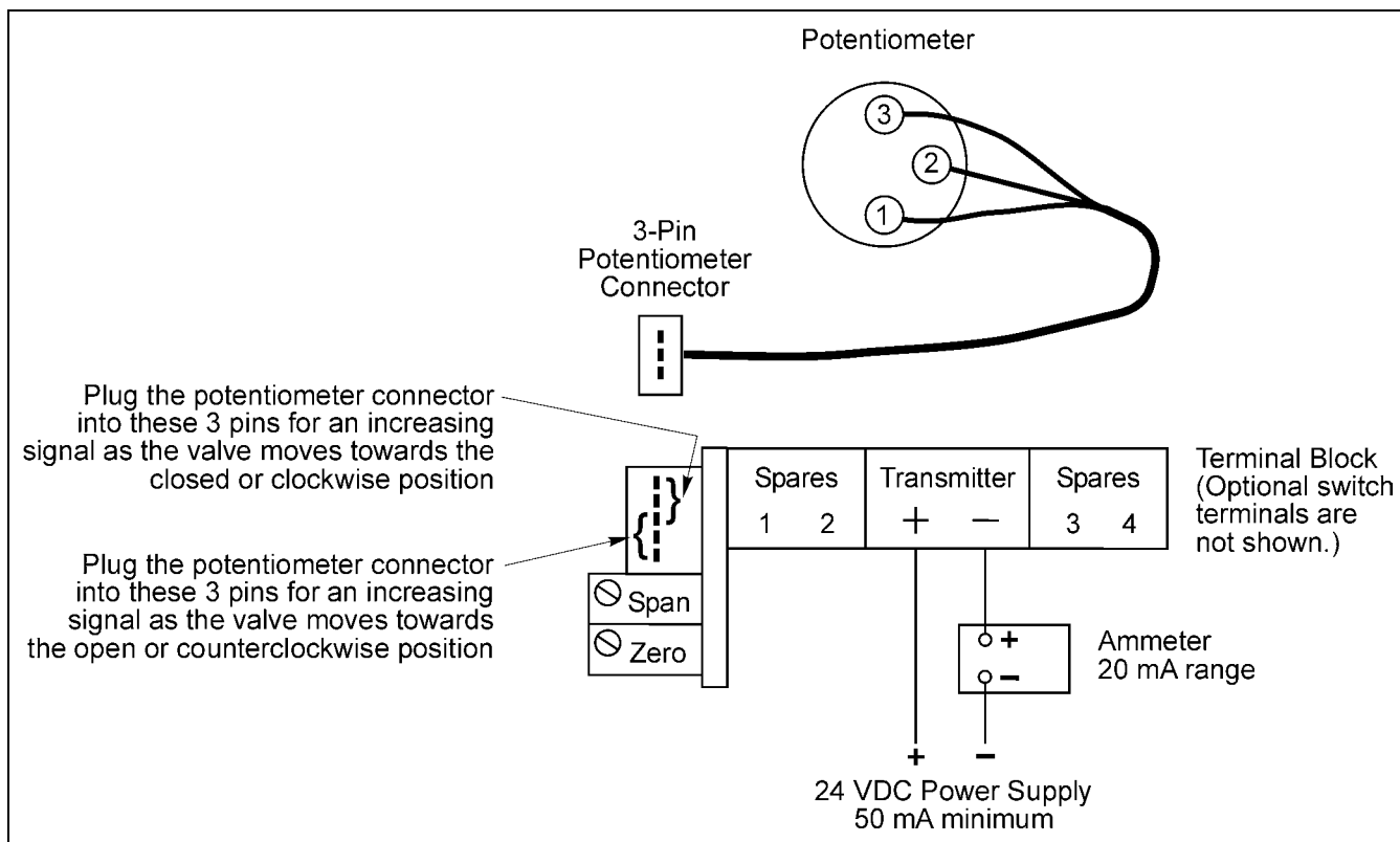
Figure 3—Position Transmitter
