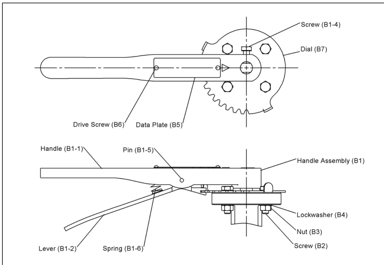
Figure 1— Parts Identification
